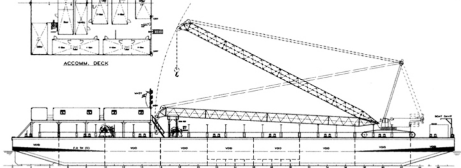
OUTBOARD PROFILE
